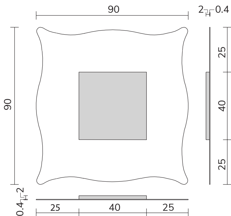
SPECCHIO VISTA RETRO / rear view mirror
