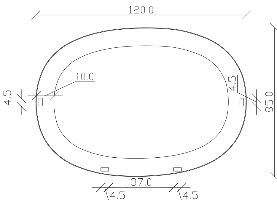
SPECCHIO VISTA RETRO / rear view mirror
